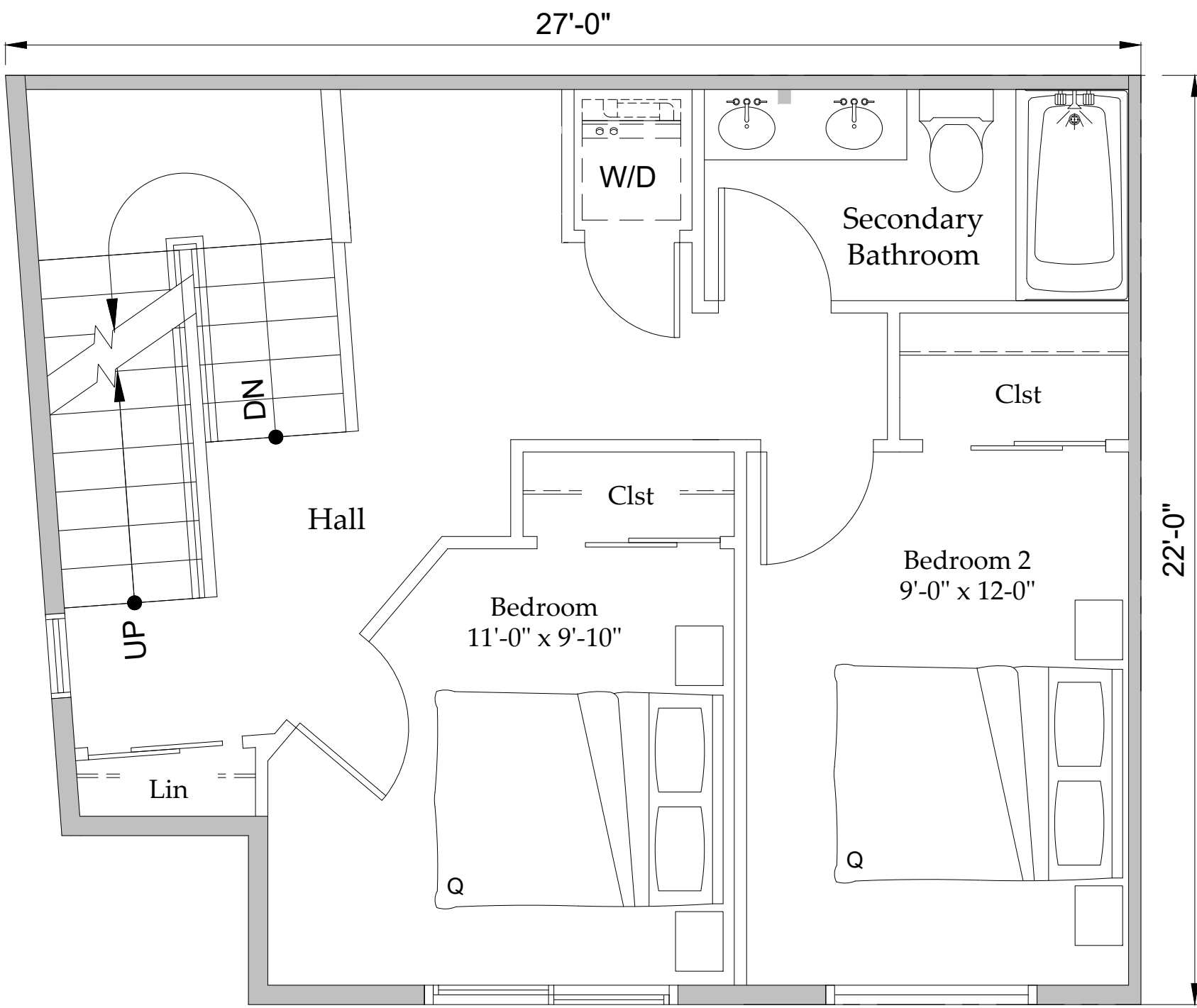
THIRD FLOOR
