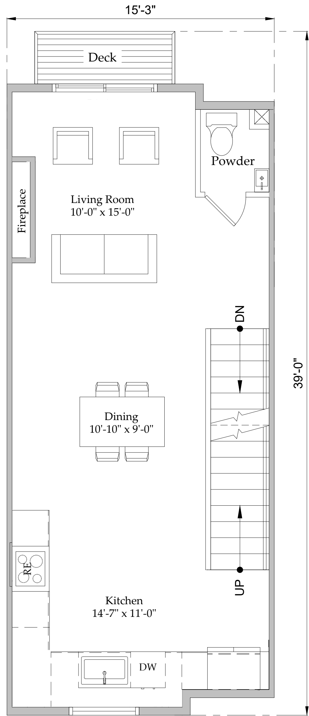
SECOND FLOOR
