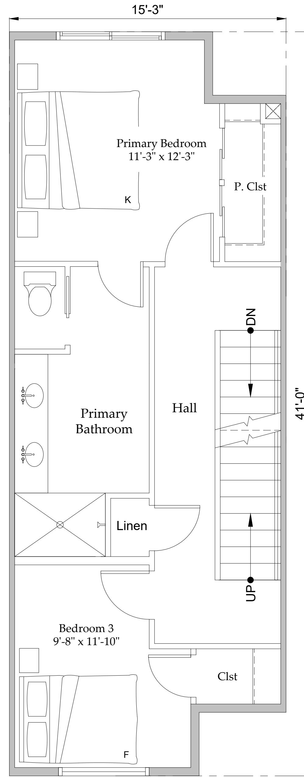
FORTH FLOOR
