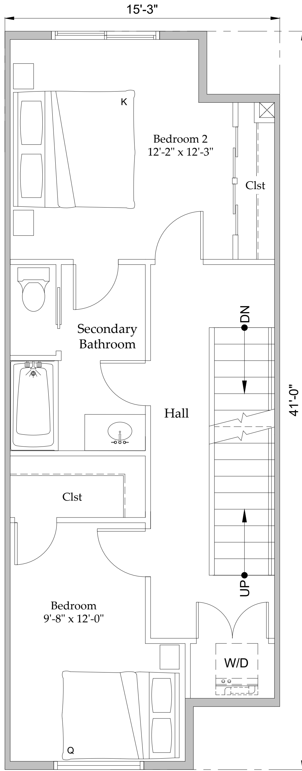
THIRD FLOOR
