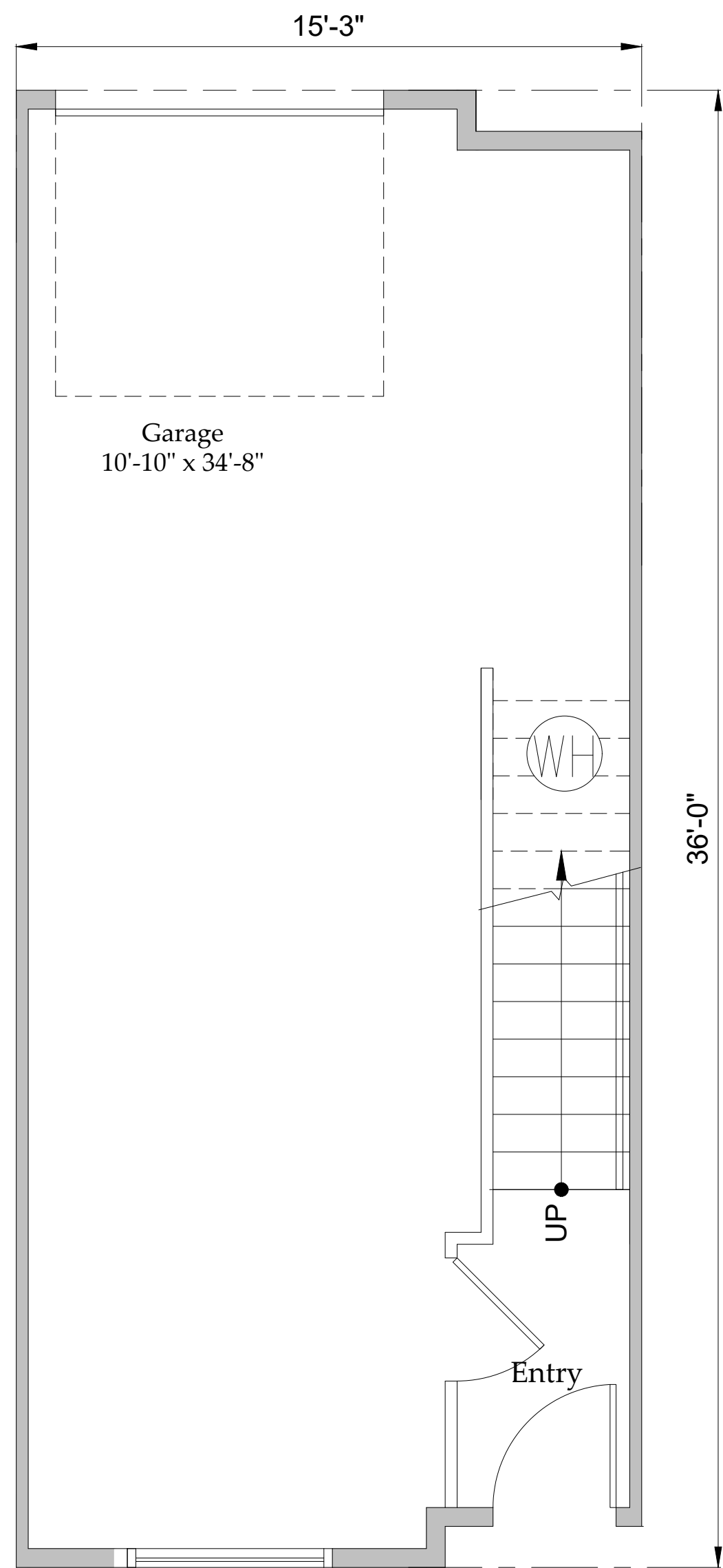
FIRST FLOOR
